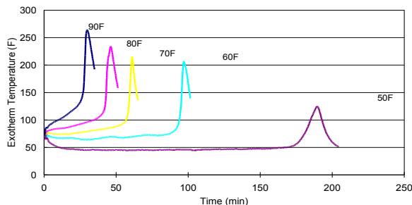
Typical Exotherm Curve for MA550 in a 30 gm Mass at Various Ambient Temperatures 5
