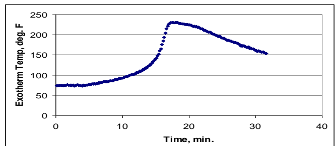
Typical Exotherm Curve for MA685 at 75°F (10 grams)
