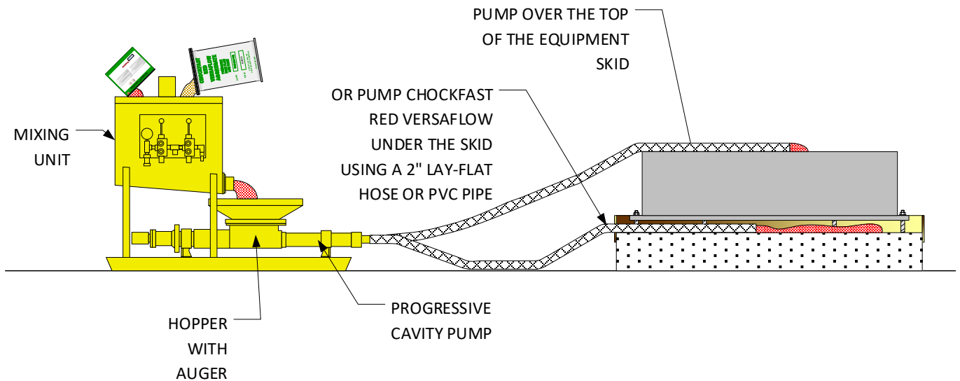
Figure 4: Placement of Grout using a Progressive Cavity Pump
