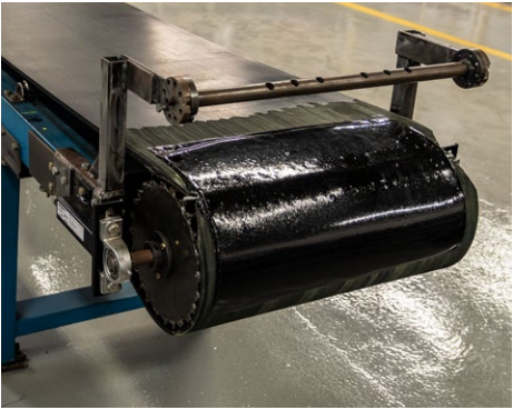
After: R-Flex® Clip Repair
